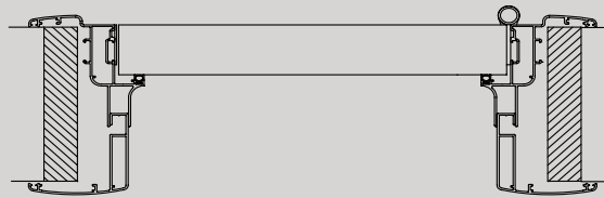
Anta tamburate sp. 43 mm / door hollow-core panels th. 43 mm
